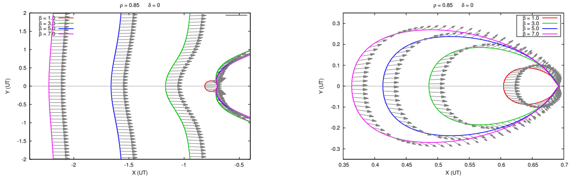
Figure 2. Family of equilibrium points for \bar{\beta} = 1, 3, 5, 7, \alpha \in [-\pi/2, \pi/2] and \delta = 0 . All the equilibria lie on the orbital plane Z = 0 . Left: Points related to L_1 , Right: Points related to L_2 . The arrows represent the normal direction to the surface of the sail at each equilibrium point.
