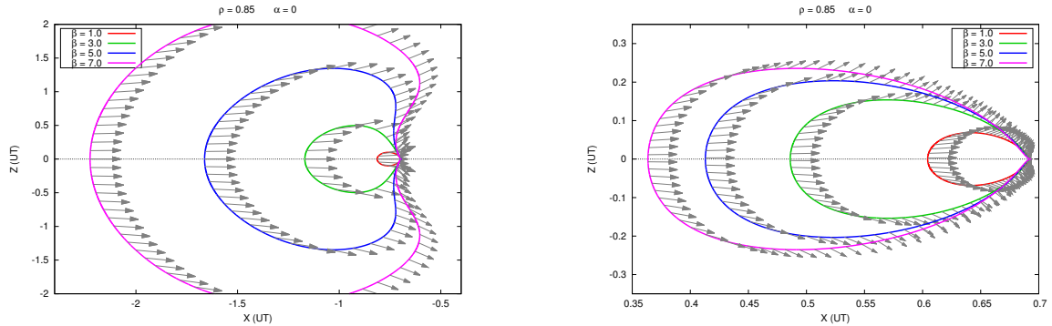
Figure 3. Family of equilibrium points for \bar{\beta} = 1, 3, 5, 7, \alpha = 0 and \delta \in [-\pi/2, \pi/2] . All the equilibria lay on the plane Y = 0 . The arrows represent the normal direction to the surface of the sail at each equilibrium point.
