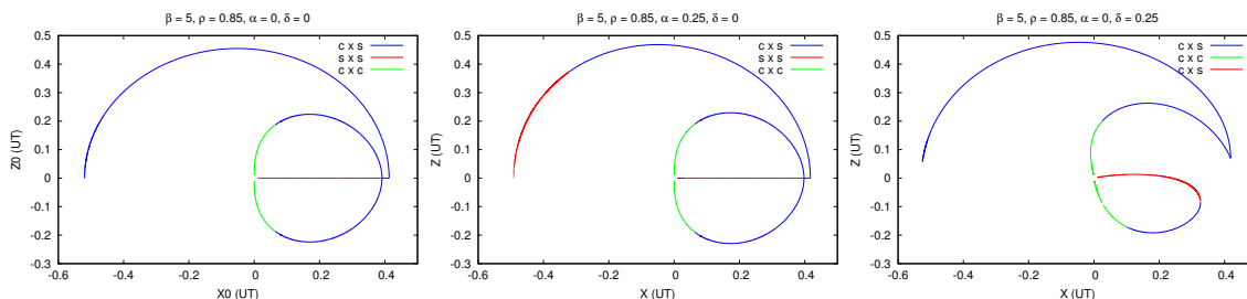
Figure 4. For \bar{\beta} = 5, \rho = 0.85, \alpha = 0, \delta = 0 left, (\alpha = 0.25, \delta = 0) middle, (\alpha = 0, \delta = 0.25) right. Continuation diagram of the families of periodic orbits on the Poincaré section \Gamma_1, x_0 vs z_0 .
