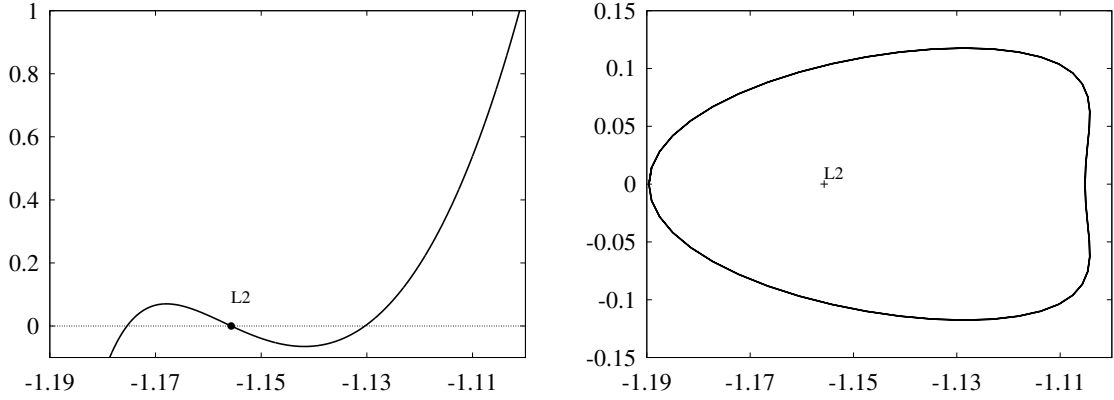
Figure 6: Left: Continuation of L_2 as a periodic orbit with respect to the mass of the Sun. Horizontal axis: x . Vertical axis: \varepsilon . See text for more details. Right: Periodic orbit near L_2 in the BCP. Horizontal axis: x . Vertical axis: y .
