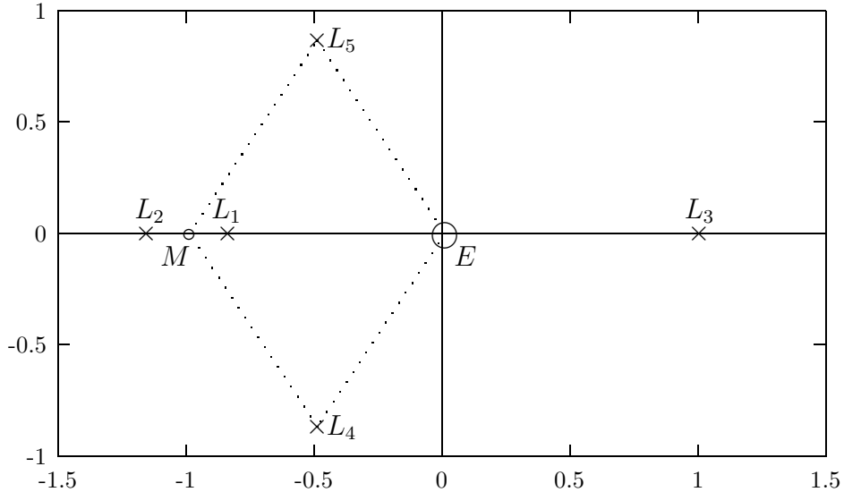
Figure 1: The Restricted Three Body Problem.
