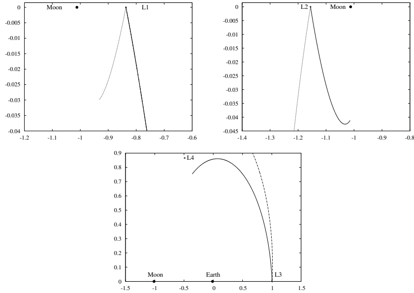
Figure 8: Approximation of order 64 of the stable (dashed) unstable (solid) manifolds of L_1 , L_2 and L_3 . Horizontal axis x . Vertical y .
