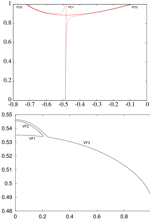
Figure 3: Left: Continuation of L_4 as a periodic orbit with respect to the mass of Sun. Horizontal axis: x . Vertical axis: \varepsilon . The black curve stands for the continuation to the BCP. The red curve for the truncated version of the BCP. See text for more details. Right: Vertical families of 2D tori for the BCP. The horizontal axis is the p_z coordinate and the vertical axis displays the frequency. See text for more details.
