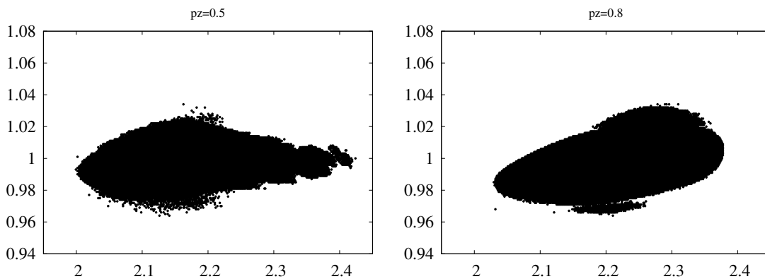
Figure 5: Stability regions with initial conditions on the tori of the VF3 identified by p_z = 0.5 and p_z = 0.8 . Horizontal axis: \alpha . Vertical axis r . See text for more details.
