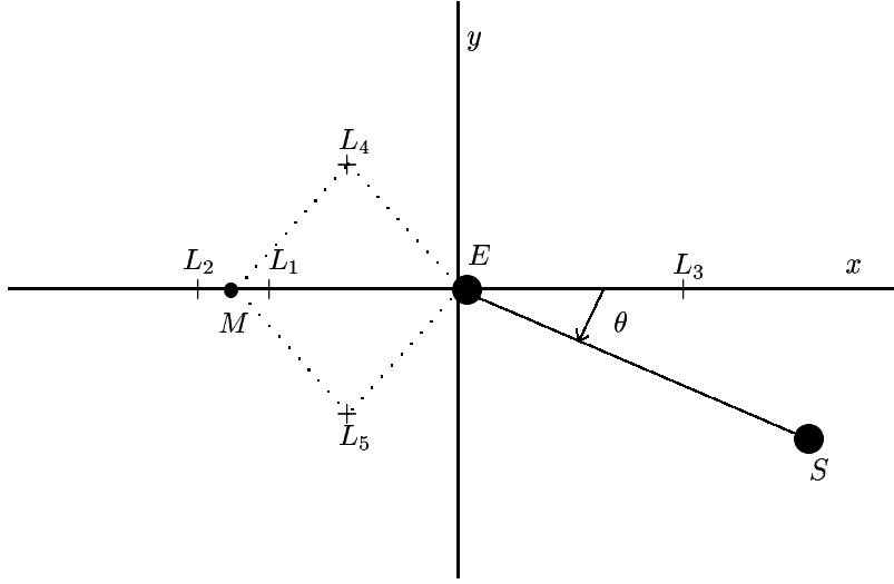
Figure 2: The Bicircular model.
