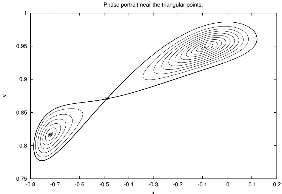
Figure 4: Stroboscopic map near the triangular points: Horizontal axis x . Vertical axis y . See text for more details.
